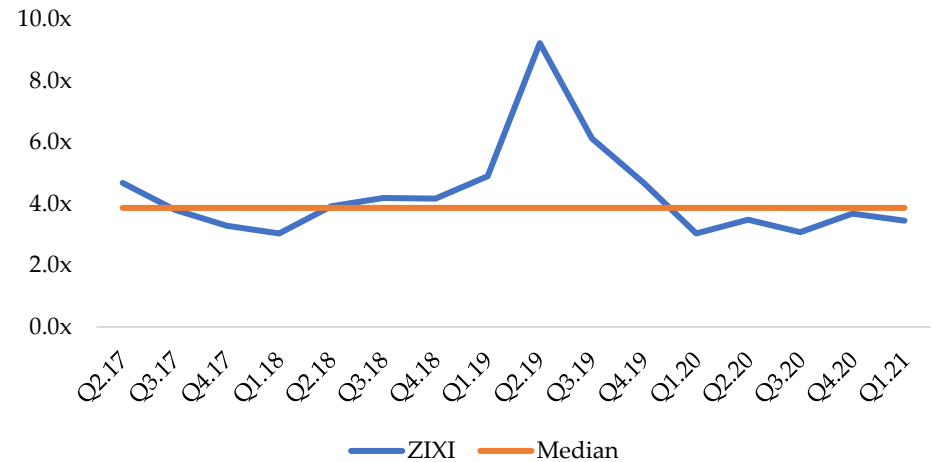
EV/Revenue Zix
