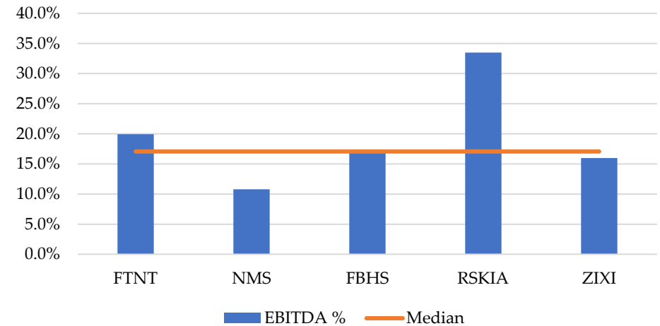
EBITDA Margin
