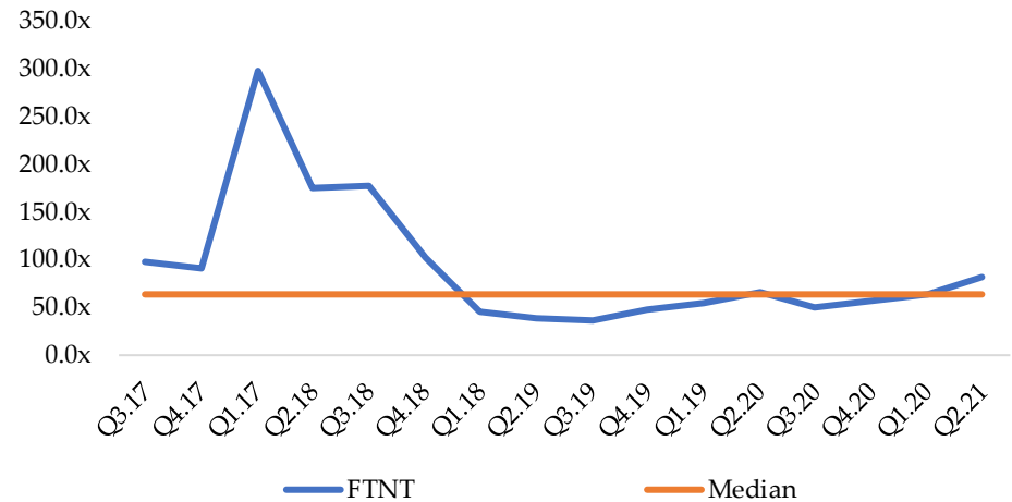
P/E Fortinet
