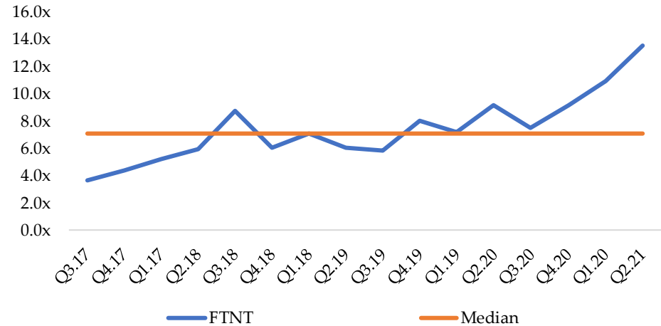
EV/Revenue Fortinet
